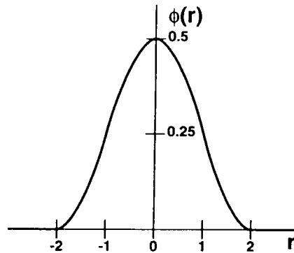
Figure 14.1. One-dimensional delta function.
